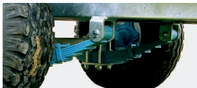
Kit balestre / Leaf springs set / Kit suspension a lames de ressort / Kit Blattfedern / Kit ballestas
